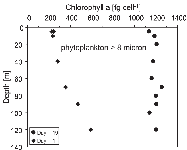
Figure 13. Amount of Chl a per cell (femtogram cell -1 ) increased about fourfold in the most stimulated largest size class ( >8 \mu\text{m} ) eukaryote phytoplankton (i.e., diatoms) during the first 19 days of the CARUSO/EisenEx experiment (data of M. J. W. Veldhuis). Such an increase of cellular Chl a was evident already from the C:Chl a ratio in one of the first bottle experiments [Coale, 1991, Figure 6] and in IronEx-2 [Cavender-Bares et al. , 1999]. In retrospect, this also indicates that Chl a exaggerates the phytoplankton biomass response to added Fe (Figures 11 and 12).
