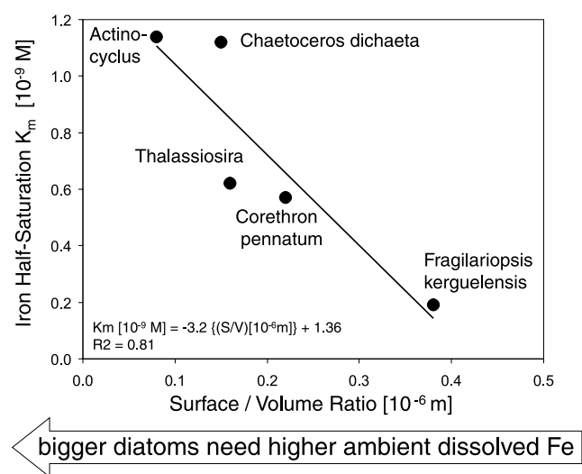
Figure 18. Inverse relationship between surface/volume ratio of medium-sized and large-sized Antarctic diatoms versus the half-saturation value K_m for growth \mu/\mu_{\max} = [\text{Fe}]/(K_m + [\text{Fe}]) after Monod [1942]. Shown are large Fragilariopsis kerguelensis and larger Corethron pennatum , Thalassiosira , and very large Actinocyclus sp., the latter very similar in perfect discoid shape and 300–400 μm size as Asteromphalus sp. [Waite and Nodder, 2001]. Graph plotted after K_m data of dissolved Fe (nM) growth curves (not shown here) in natural Antarctic seawater; see Timmermans et al. [2004] for these growth curves.
